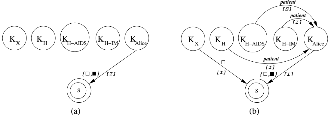
Figure 3: (a) Automaton representing the configurations S = \{\langle K_{Alice}, \square \rangle, \langle K_{Alice}, \blacksquare \rangle\} . (b) Automaton representing the configurations in pre^*(S) .
