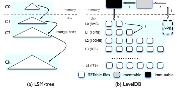
Figure 1: LSM-tree and LevelDB Architecture. This figure shows the standard LSM-tree and LevelDB architecture. For LevelDB, inserting a key-value pair goes through many steps: (1) the log file; (2) the memtable; (3) the immutable memtable; (4) a SSTable in L0; (5) compacted to further levels.
