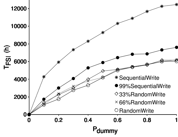
Fig. 4. T_{FSI} with workloads of different percentage of random and sequential writes without FTL.
