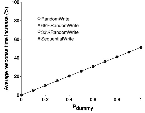
Fig. 5. Average response time (ms) with workloads of different percentage of random and sequential write requests.
