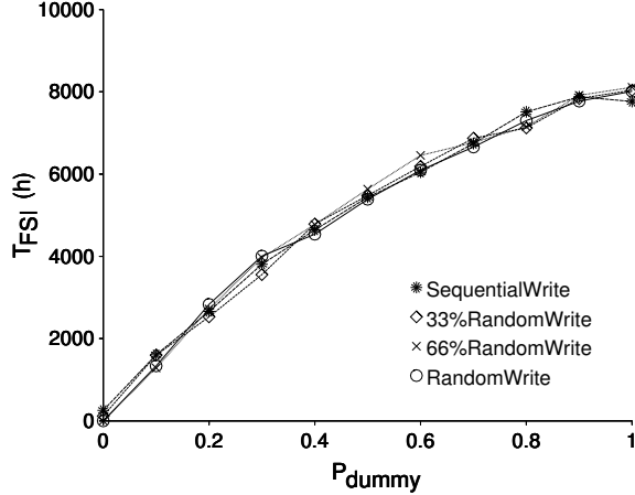
Fig. 2. T_{FSI} with workloads of different percentage of random and sequential writes with wear-leveling FTL.
