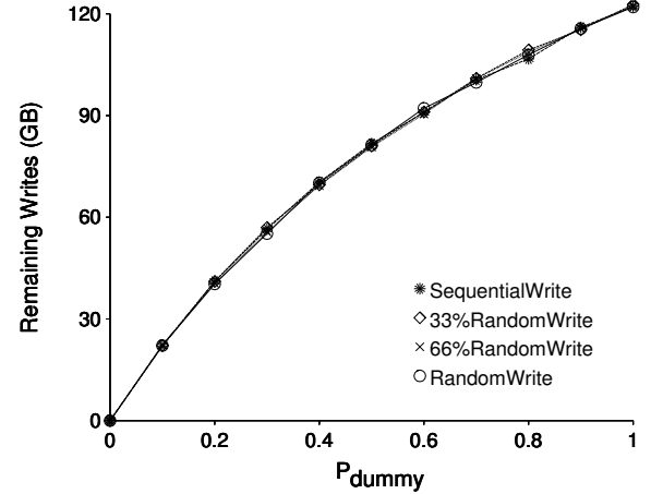
Fig. 3. Remaining writes on the surviving drive with workloads of different percentage of random and sequential writes with wear-leveling FTL.
