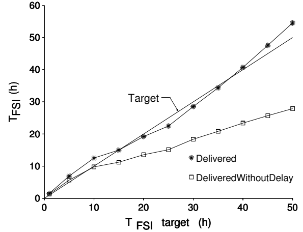
Fig. 9. Delivered T_{FSI} with and without delay with different target T_{FSI} (random workload).
