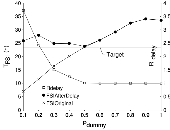
Fig. 6. Effect of adding delay in degraded period to adjust T_{FSI} when P_{dummy} is not accurate.
