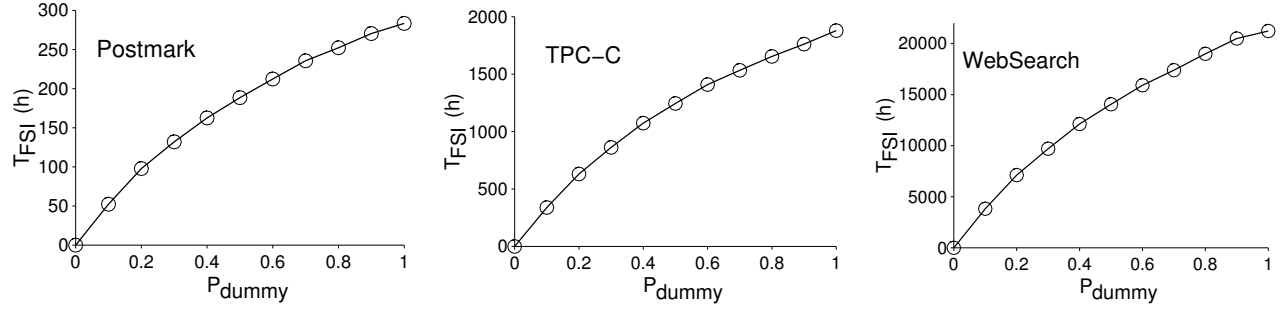
Fig. 10. T_{FSI} for the Postmark, TPC-C, and WebSearch traces with different dummy write frequencies.
