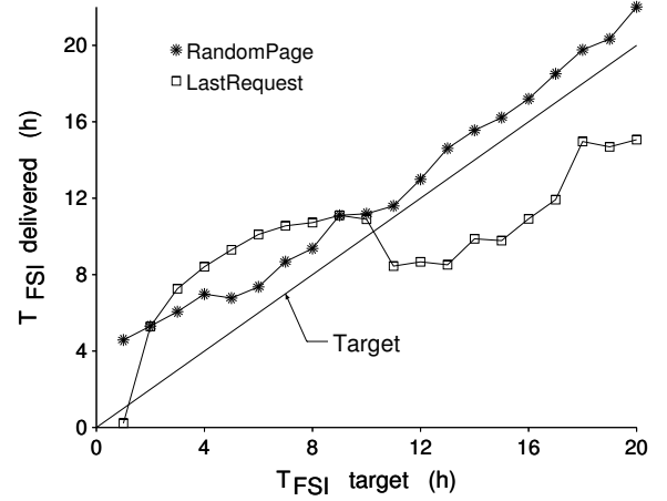
Fig. 7. Delivered T_{FSI} using dummy write page chosen at random and as last request page.
