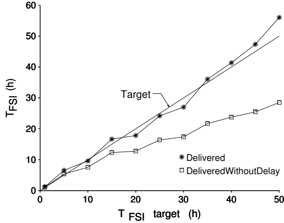
Fig. 8. Delivered T_{FSI} with and without delay with different target T_{FSI} (sequential workload).
