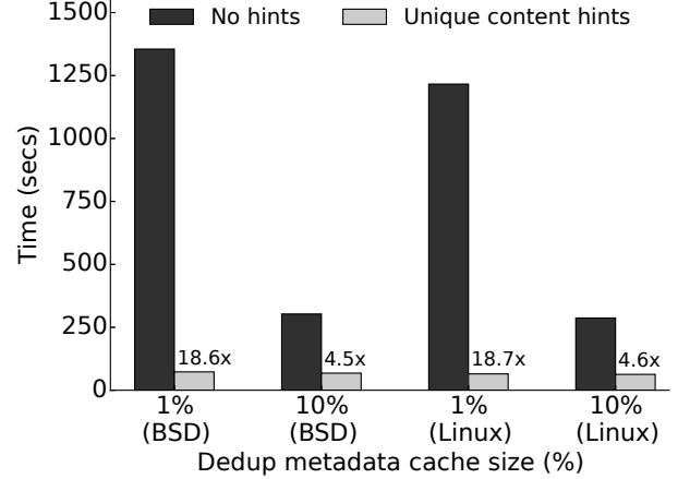
Figure 9: File Encryption Results. The numbers on top of the light colored bars show the speedup achieved for the file encryption workload when run with unique content hints on iDedup.
