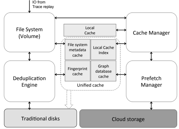
Figure 7: Cloud Gateway Simulator.
