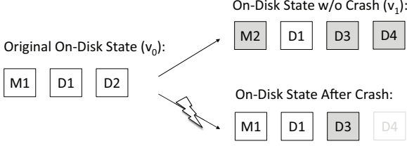
Figure 1: A Crash in Ext4 Ordered Mode. This image shows a file whose data is rendered inconsistent by a crash in ext4 ordered mode. The original state of the file on disk ( v_0 ) is shown at left, with its inode block, M1 , pointing to two data blocks, D1 and D2 . An application then overwrites the last block ( D2 ) with D3 and appends a new block, D4 , resulting in an updated inode block, M2 . If there is no crash, the final state of the file will be v_1 , as shown in the upper right. All newly written blocks are marked with gray. If a crash occurs before M2 is journaled but after D3 and D4 are written, the file will be in an inconsistent state after recovery, as shown in the lower right.
