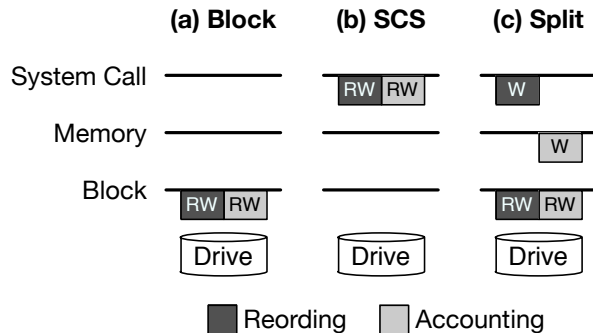
Figure 2: Scheduling Architectures. The boxes show where scheduler hooks exist for reordering I/O requests or doing accounting. Sometimes reads and writes are handled differently at different levels, as indicated by “R” and “W”.
