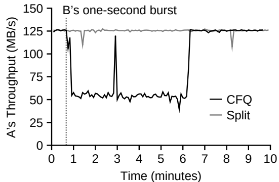
Figure 1: Write Burst. B’s one-second random-write burst severely degrades A’s performance for over five minutes. Putting B in CFQ’s idle class provides no help.
