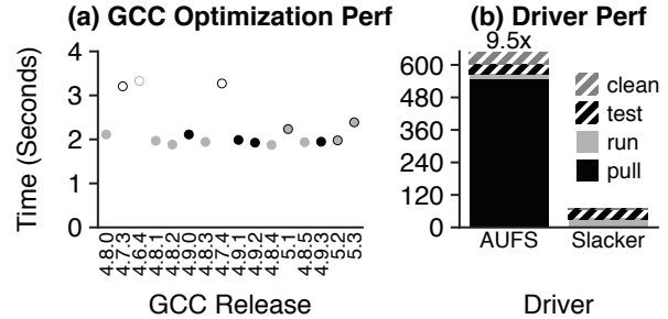
Figure 24: GCC Version Testing. Left: run time of a C program doing vector arithmetic. Each point represents performance under a different GCC release, from 4.8.0 (Mar ‘13) to 5.3 (Dec ‘15). Releases in the same series have a common style (e.g., 4.8-series releases are solid gray). Right: performance of MultiMake is shown for both drivers. Time is broken into pulling the image, running the image (compiling), testing the binaries, and deleting the images from the local daemon.
