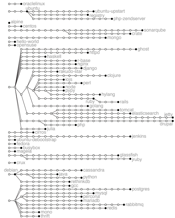
Figure 3: HelloBench Hierarchy. Each circle represents a layer. Filled circles represent layers tagged as runnable images. Deeper layers are to the left.
