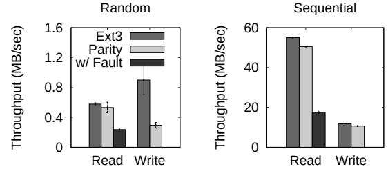
Figure 11: Parity Throughput. The figure plots the throughput of the parity policy under some simple microbenchmarks. For sequential writes, we simply write 24 MB to disk. For random reads and writes, we either read or update random 4-KB blocks in a large (2 GB) file. For reads, both the normal and failure cases are reported; failures are injected by causing each initial read to fail which triggers reconstruction. Each experiment is repeated 60 times; averages and standard deviations are reported.
