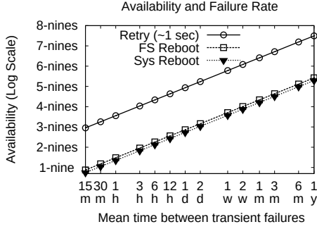
Figure 9: Reboot vs. Retry (Availability). The graph shows the computed availability (in terms of “nines”) plotted versus the mean time between transient failures for the three policies: full system reboot, file system reboot, and retry. The system is considered “available” when its delivered performance is within 10% of average steady-state performance.
