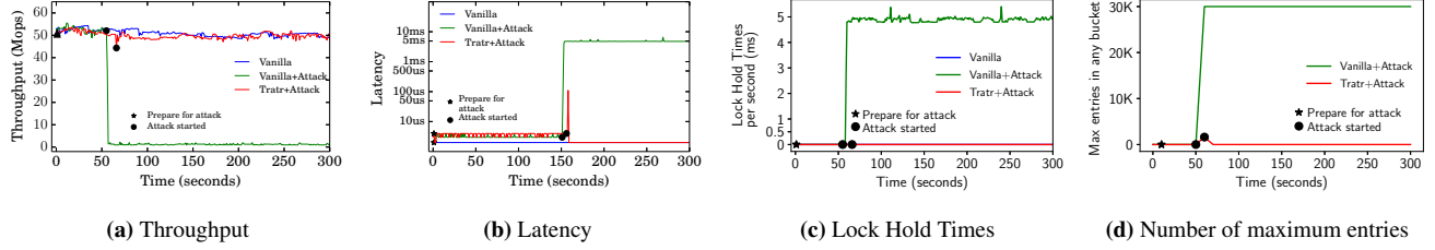
Figure 6: FT benchmark performance without attack, with attack and with Trätr. (a) Timeline of the throughput showing the impact on the throughput due to the attack for the Vanilla and Trätr kernel. (b) Timeline of the average latency of the time to release the lock measured using systemtap for a similar experiment. (c) Timeline of the lock hold times of the victim for Vanilla and Trätr kernel. (d) Timeline of the maximum number of entries of the attacker in any bucket for Vanilla and Trätr kernel.
