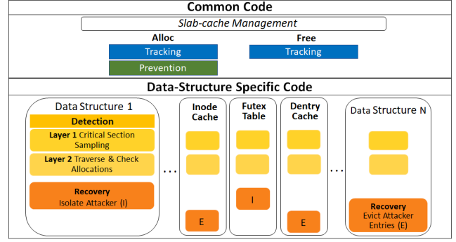
Figure 2: High-level design of Trätr. Design showing the four mechanisms of Trätr. The Tracking and Prevention mechanisms are part of slab-cache management. Layer 1 Detection measures the synchronization stalls to indirectly measure long critical sections. On finding longer stalls, Trätr triggers layer two checks if a user has a majority of object allocations. On finding one, Trätr identifies that user as an attacker and initiates prevention and recovery mechanisms. The prevention mechanism prevents the attacker from allocating more entries. Depending on the type of data structure, an appropriate recovery is initiated. The upper box shows the common code, while the lower box shows data structure-specific code.
