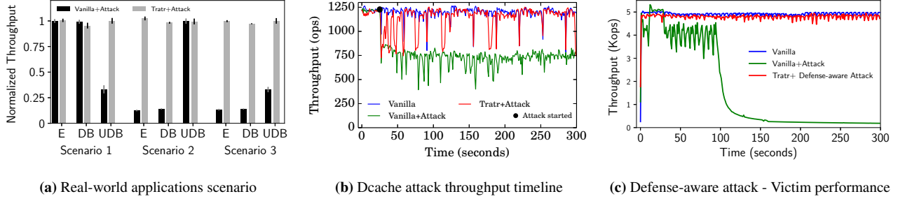
Figure 8: Performance comparison of the various applications across different scenarios. Performance comparison of Vanilla and Trätr with and without attack when subjected to different attack scenarios. (b) Timeline of throughput showing impact on the throughput due to the dcache attack for the Vanilla and Trätr kernel. (c) Throughput timeline for the inode cache attack highlighting the victim’s performance.
