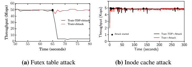
Figure 7: Performance of Trätr components. Throughput timeline for the futex and inode cache attacks explaining the importance of detection, prevention and recovery. We also show the timeline for Trätr-TDP. Trätr-TDP denotes the kernel version that has the tracking, detection and prevention mechanisms enabled.
