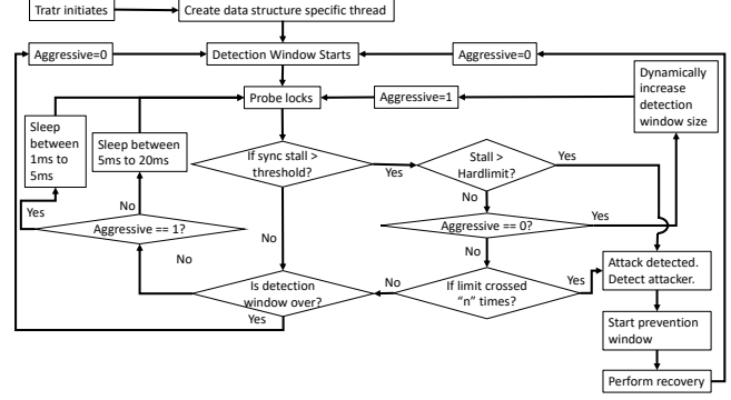
Figure 3: Flowchart of the kernel thread associated with a data structure.
