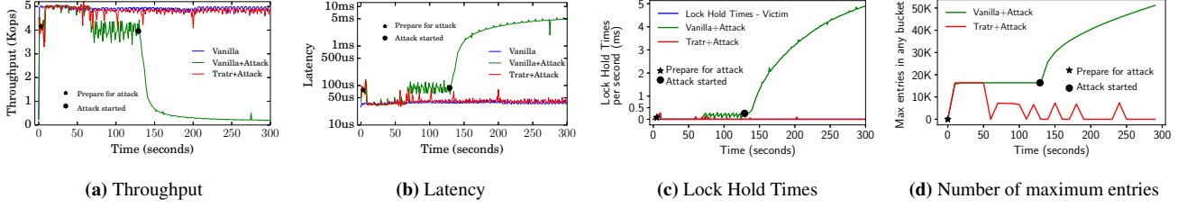
Figure 5: IC benchmark performance without attack, with attack and with Trätr. (a) Timeline of the throughput showing the impact on the throughput due to the attack for the Vanilla and Trätr kernel. With Trätr, the attacker is not able to launch an attack. (b) Timeline of the average latency showing the time to create the file. (c) Timeline of the lock hold times of the victim for Vanilla and Trätr kernel. (d) Timeline of the maximum number of entries of the attacker in any bucket for Vanilla and Trätr kernel.
