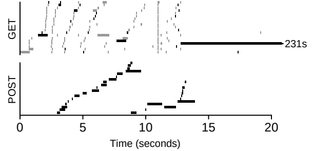
Figure 3: Google Gmail. Black bars represent RPC messages; gray bars represent other messages. The bar ends represent request and response times. The bars are grouped as POSTs and GETs; vertical positioning is otherwise arbitrary.
