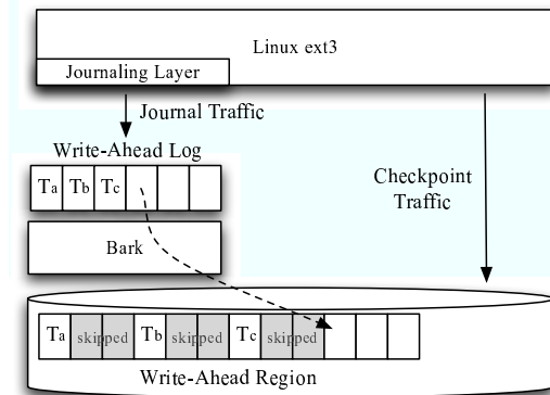
Figure 12: Bark-itecture. The figure illustrates how a file system can be mounted upon Bark to improve journal write performance. All journal traffic is directed through Bark, which picks a skip distance based on think time and the position of the last write to disk. Bark performs this optimization transparently, thus improving the performance of journal writes with no change to the file system above. In the specific example shown, the file system has committed three transactions to disk: Ta, Tb, and Tc. Bark, using its performance model, has spread the transactions across the physical disk, leaving empty spaces (denoted as “skipped”) in the write-ahead region.
