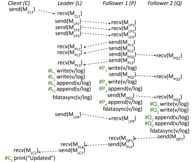
Figure 2: ZooKeeper protocol for an update workload. The figure shows the sequence of steps when the client interacts with the ZooKeeper cluster. The workload updates a value. The client prints to stdout once the update request is acknowledged.
