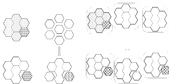
Figure 2: Sensible-boundary identification mechanisms. The figure illustrates some methodologies that can be used to identify the optimal boundaries to enforce; the concurrent server is imagined to be composed of separable hexagons, and the shaded hexagons represent faulting components. In the optimistic approach, the system is allowed to fault once and the culprit component is isolated in future; in the pessimistic approach, all components are isolated at first and the trusted components are later combined; finally, the cooperative approach collects information from multiple systems to decide on what to isolate.
