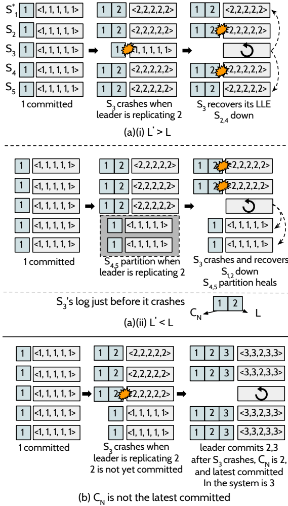
Figure 4: LLE Recovery. The figure shows how L' may not be equal to L . For each node, we show its log and LLE-MAP . The leader ( S_1 ) is marked *; crashed nodes are annotated with a crash symbol; nodes partitioned are shown in a dotted box; epochs are not shown.
