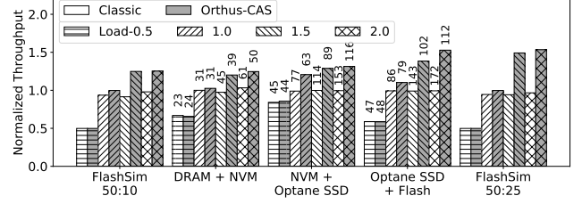
Figure 3: Orthus-CAS on Various Hierarchies. The figure shows NHC's performance under read-only workloads (95% hit rates) with different amounts of load. We use the same devices as in Figure 1. We also use FlashSim to simulate devices with different performance characteristics. Load-1.0 is specified as the minimum load to reach full cache-device read bandwidth; Load-0.5, 1.5, and 2.0 are created by scaling Load-1.0. All throughputs are normalized to the maximum read bandwidth of the caching device. Latency ( \mu\text{s} ) is shown above each bar (not comparable across hierarchies).
