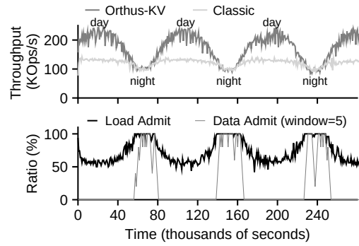
Figure 4: Orthus-KV With ZippyDB workloads. This figure shows the Orthus-KV throughput (top) as well as load/data admit ratios over time in Orthus-KV (bottom). We focus on the hierarchy of Optane/Flash. The Facebook ZippyDB benchmark generates key-value operations based on realistic trace statistics; the request rate models the diurnal load sent to ZippyDB servers. We speed up the replay by 1000 to stress the storage system and to better evaluate NHC's reactions to shifting loads.
