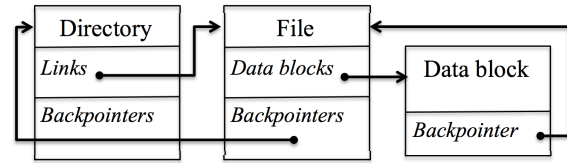
Figure 1: Backpointers. The figure shows a conceptual view of the backpointers present in NoFS. The file has a backpointer to the directory that it belongs to. The data block has a backpointer to the file it belong to. Files and directories have many backpointers while data blocks have a single backpointer.
