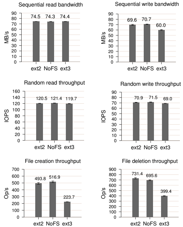
Figure 4: Micro-benchmark performance. This figure compares file-system performance on various micro-benchmarks. The sequential benchmarks involve reading and writing a 1 GB file. The random benchmarks involve 10K random reads and writes in units of 4088 bytes (4096 bytes - 8 byte backpointer) across a 1 GB file, with a fsync after 1000 writes. The creation and deletion benchmarks involve 100K files spread over 100 directories, with a fsync after every create or delete.
