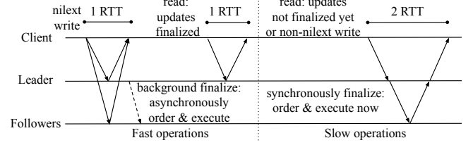
Figure 2. Nilext-aware Replication. The figure shows how a nilext-aware replication protocol handles different operations.
