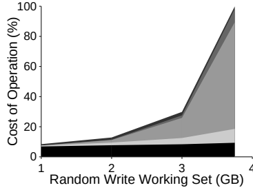
Figure 8: Nameless FTL Utilization. Break down of device utilization with the nameless FTL under random writes of different ranges.
