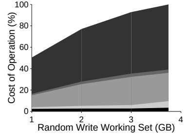
Figure 9: Hybrid FTL Utilization. Break down of device utilization with the hybrid FTL under random writes of different ranges.
