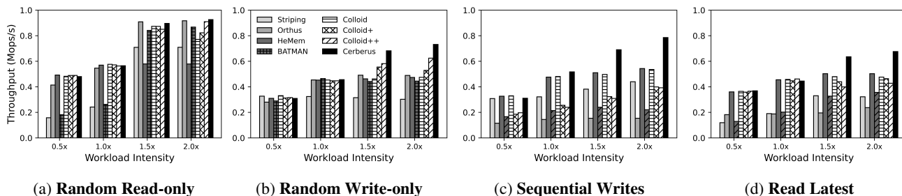
Figure 4: Static Workload. The workload is running on the Optane/NVMe hierarchy with 750GB working set. In (a), under intensity 2.0 \times , Colloid, Colloid+, Colloid++, Cerberus migrate 134GB, 122GB, 62GB, 50GB of data in total. In (b), under intensity 2.0 \times , Colloid, Colloid+, Colloid++, Cerberus migrate 0GB, 93GB, 80GB, 65GB of data in total.
