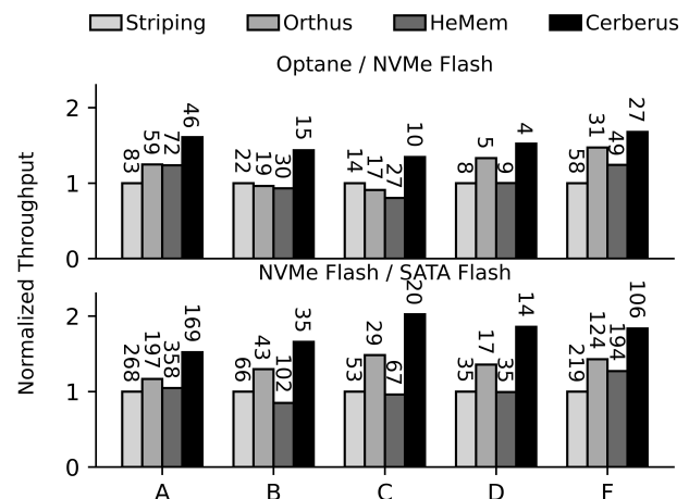
Figure 11: YCSB. CacheLib uses the default parameters from CacheBench with 4GB DRAM cache. All the workloads are Zipfian ( \theta = 0.8 ) with 1KB values and 16-byte keys running under 256 threads with 20M records. The cache throughput is normalized to the throughput of the default (striping) system and the number above each bar is P99 latency in microseconds. Workload E is excluded due to CacheLib's lack of support for range queries.
