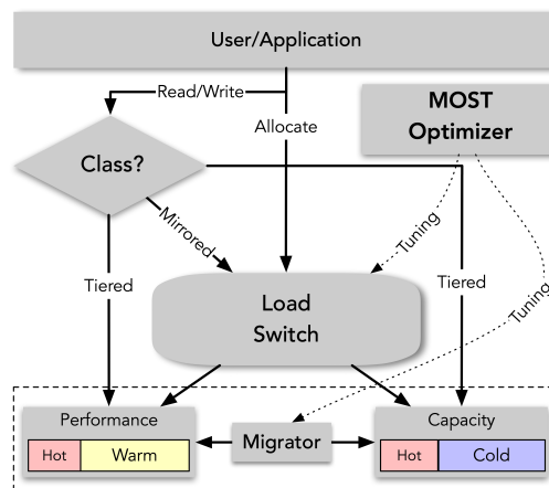
Figure 2: MOST Architecture.
