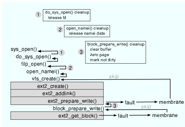
Figure 4: The Skip/Trust Unwind Protocol. The figure depicts the call path from the open() system call through the ext2 file system. The first sequence of calls (through vfs_create() ) are in the generic (trusted) kernel; then the (untrusted) ext2 routines are called; then ext2 calls back into the kernel to prepare to write a page, which in turn may call back into ext2 to get a block to write to. Assume a fault occurs at this last level in the stack; Membrane catches the fault, and skips back to the last trusted kernel routine, mimicking a failed call to ext2_get_block() ; this routine then runs its normal failure recovery (marked by the circled “3” in the diagram), and then tries to return again. Membrane’s control-flow capture machinery catches this and then skips back all the way to the last trusted kernel code ( vfs_create ), thus mimicking a failed call to ext2_create() . The rest of the code unwinds with Membrane’s interference, executing various cleanup code along the way (as indicated by the circled 2 and 1).
