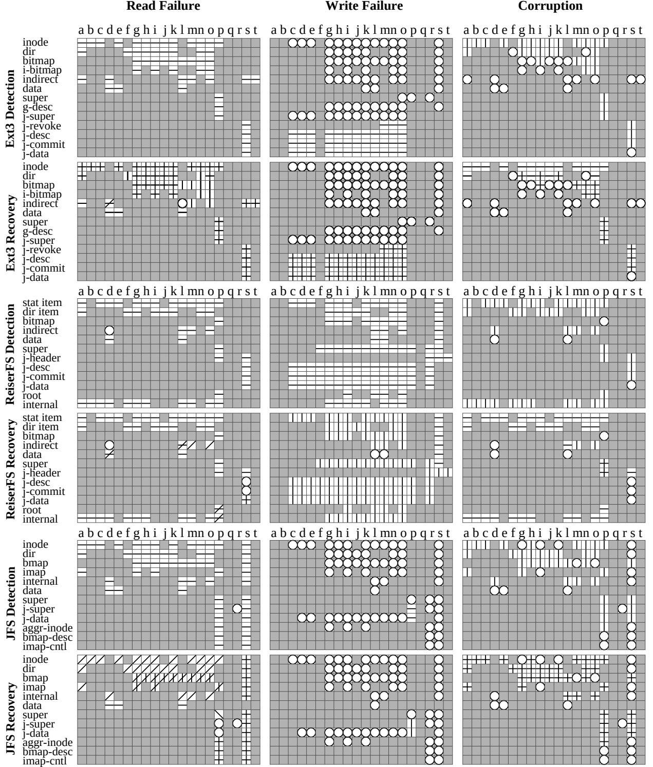
Figure 2: File System Failure Policies. The tables indicate both detection and recovery policies of ext3, ReiserFS, and JFS for read, write, and corruption faults injected for each block type across a range of workloads. The workloads are a : path traversal b : access, chdir, chroot, stat, statfs, lstat, open c : chmod, chown, utimes d : read e : read-link f : getdirentries g : creat h : link i : mkdir j : rename k : symlink l : write m : truncate n : rmdir o : unlink p : mount q : fsysnc, sync r : umount s : FS recovery t : log write operations. A gray box indicates that the workload is not applicable for the block type. If multiple mechanisms are observed, the symbols are superimposed.
