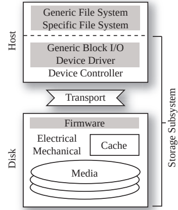
Figure 1: The Storage Stack. We present a schematic of the entire storage stack. At the top is the file system; beneath are the many layers of the storage subsystem. Gray shading implies software or firmware, whereas white (unshaded) is hardware.
