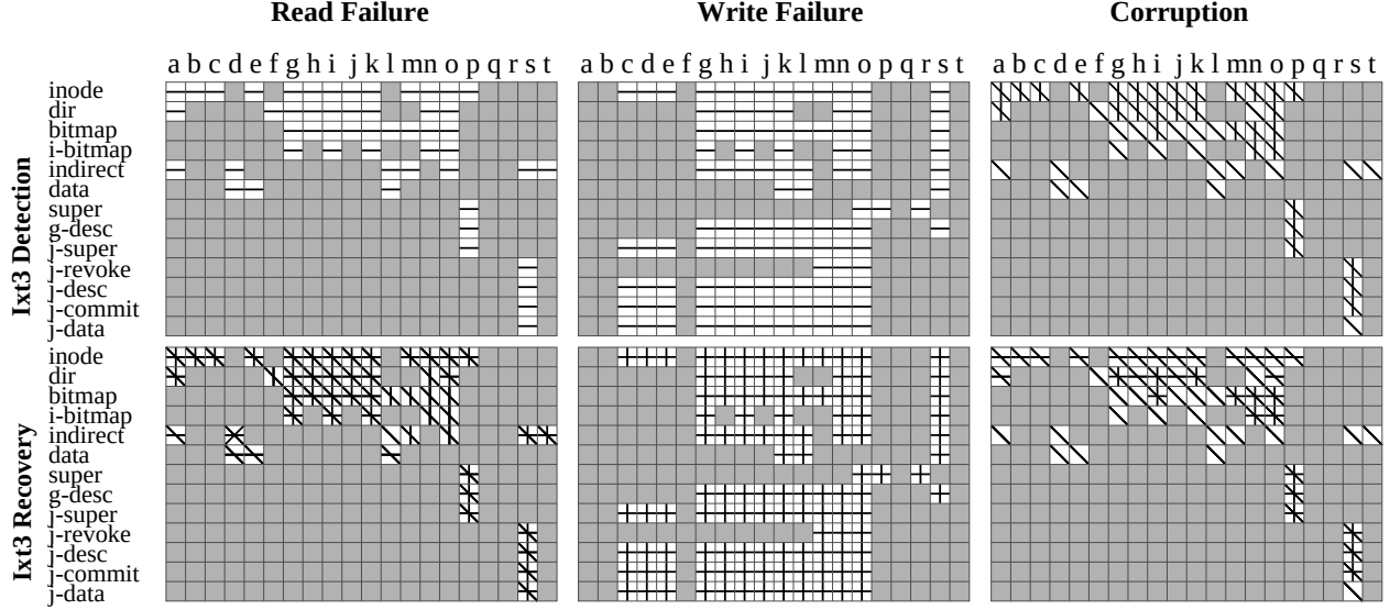
Figure 3: Ixt3 Failure Policy. The tables plot both detection and recovery policies of ixt3 for read, write, and corruption faults injected for each block type across a range of workloads. The workloads are varied across the columns of the figure, and the different block types of the ixt3 file system are varied across the rows. The workloads are grouped in the same manner as in Figure 2.
