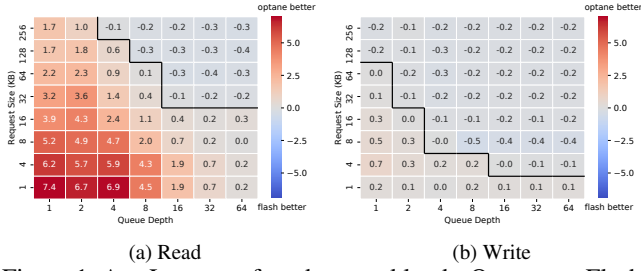
Figure 1: Avg Latency of random workloads, Optane vs. Flash
