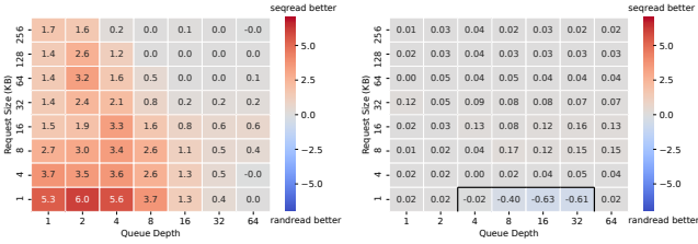
(a) Flash-based SSD (b) Optane 905P SSD Figure 4: Avg Read Latency Random vs. Sequential
