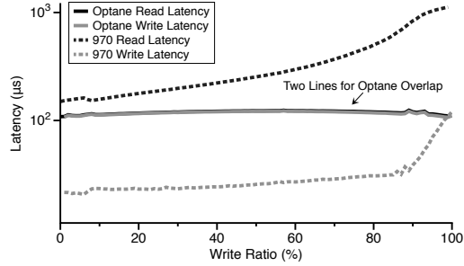
Figure 7: Latency of Mixed Reads and Writes
