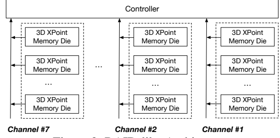
Figure 2: RAID-like Architecture
