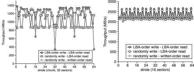
(a) Flash-based SSD (b) Optane 905P SSD Figure 11: Detecting Mapping Policy
