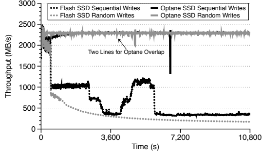
Figure 10: Throughput of Sustained Writes
