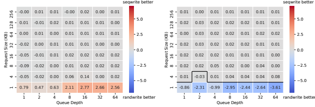
(a) Flash-based SSD (b) Optane 905P SSD Figure 5: Avg Write Latency Random vs. Sequential
