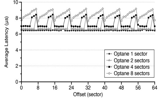
Figure 9: Identifying Influence of Misalignment
