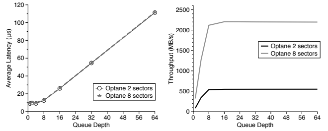
(a) Latency (b) Throughput Figure 8: Performance of Small Requests
