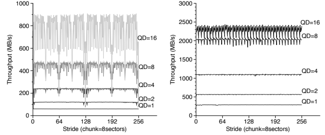
(a) Flash SSD (b) Optane 905P SSD Figure 3: Detecting Interleaving Degree
