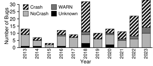
Figure 1. Number of deterministic bugs by the year. Examples of NoCrash consequences include data corruption, performance issue, permission issue, freeze, deadlock, etc.
