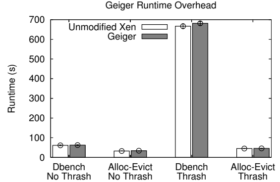
Figure 8. Geiger Runtime Overhead. The figure shows that Geiger imposes very small runtime overheads for two workloads that stress its inference heuristics.
