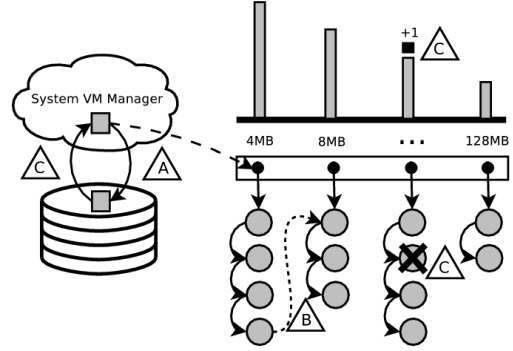
Figure 9. MemRx Operation. The figure shows a schematic of the cache simulation implemented by MemRx. A) When a page is evicted by a guest, this event is detected by Geiger and an entry is added to the head of a series of queues. B) If necessary, queue entries ripple from the tail of one queue to the head of the next. C) Upon reload, the associated queue entry is removed and an array entry associated with that queue is incremented. Each entry tracks which sub-queue it appears in to enable fast depth estimation.
