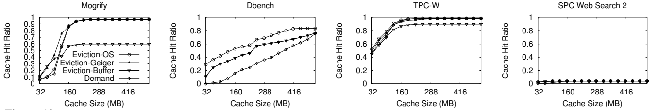
Figure 13. Secondary Cache Hit Ratio. The figure compares the cache hit ratio in a secondary storage cache for various workloads when demand placement (Demand), eviction placement based on inferred evictions (Eviction-Buffer and Eviction-Geiger), and eviction placement based on actual evictions (Eviction-OS) is used. Experiments are performed using cache sizes from 32 MB to 512 MB.
