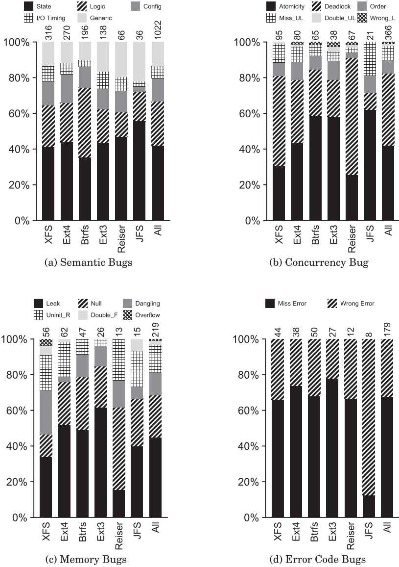
Fig. 9. Detailed bug patterns. The detailed classification for each bug pattern; total number of bugs is shown on top of each bar.
