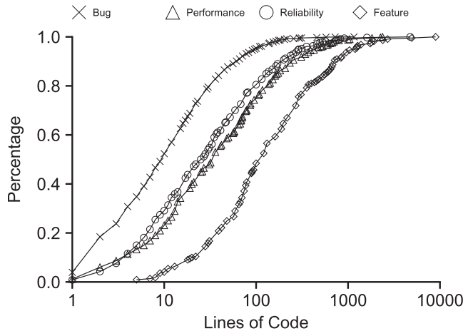
Fig. 3. Patch size. This figure shows the size distribution for different patch types, in terms of lines of modifications. The x-axis shows the lines of code in log scale; the y-axis shows the percentage of patches.
