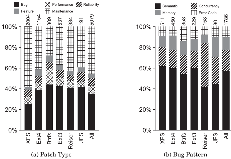
Fig. 2. Patch type and bug pattern. This figure shows the distribution of patch types and bug patterns. The total number of patches is on top of each bar.
