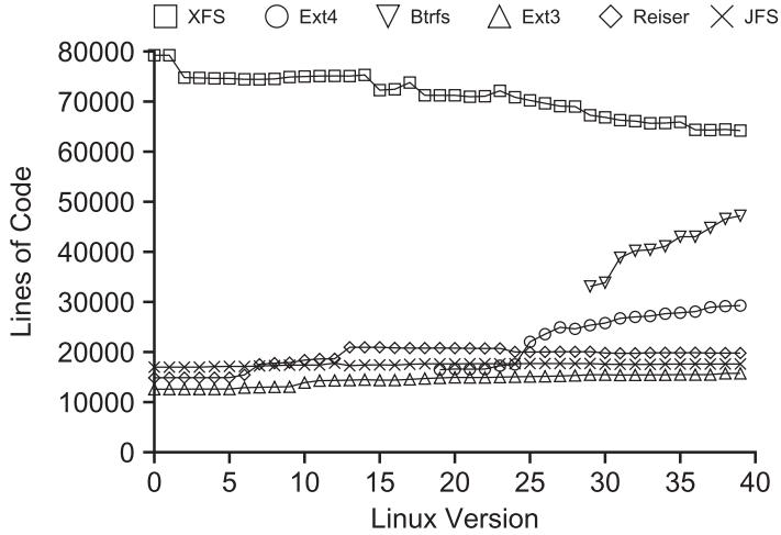
Fig. 5. File-system code evolution. This figure shows the lines of code for each file system in Linux 2.6 series. The x-axis shows 40 versions of Linux 2.6; the y-axis shows lines of code (LOC). Note that LOC of Ext3 includes the code of JBD and LOC of Ext4 includes the code of JBD2.
