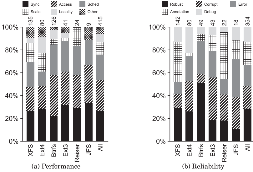
Fig. 10. Performance and reliability patches. This figure shows the performance and reliability patterns. The total number of patches is shown on top of each bar.
