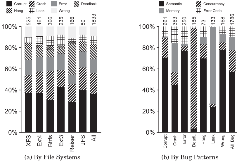
Fig. 8. Bug consequences. This figure displays the breakdown of bug consequences for file systems and bug patterns. The total number of consequences is shown on top of each bar. A single bug may cause multiple consequences; thus, the number of consequences instances is slightly higher than that of bugs in Figure 2(b).
