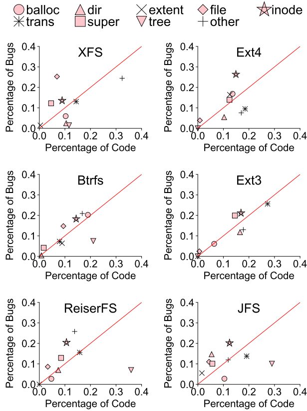
Fig. 6. File-system code and bug correlation. This figure shows the correlation between code and bugs. The x-axis shows the average percent of code of each component (over all versions); the y-axis shows the percent of bugs of each component (over all versions).
