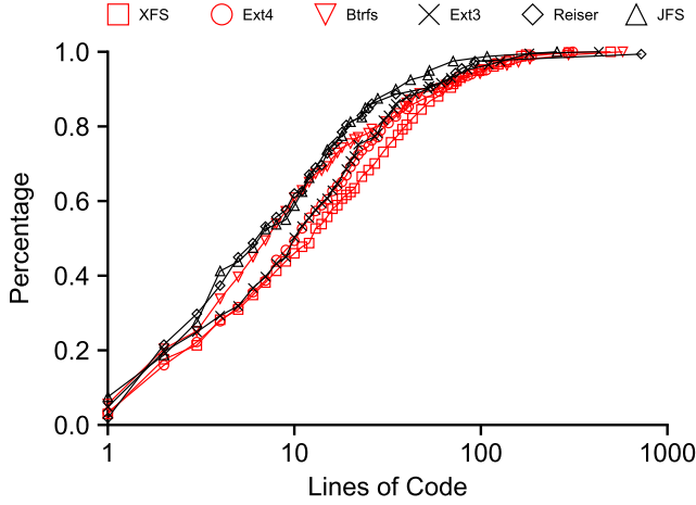
Fig. 4. Bug patch size. This figure shows the size distribution of bug patches for different file systems, in terms of lines of modifications. The x-axis shows the lines of code in log scale; the y-axis shows the percentage of patches.
