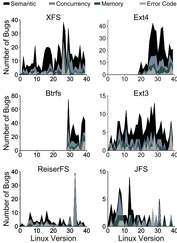
Fig. 7. Bug pattern evolution. This figure shows the bug pattern evolution for each file system over all versions.
