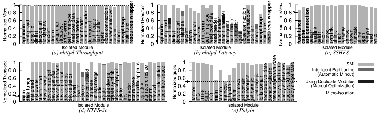
Figure 4: Partitioned Performance. Performance of different configurations normalized to the performance of the unmodularized application is shown. Module names are shown within the bars. Modules with bold names do not possess some capability.
