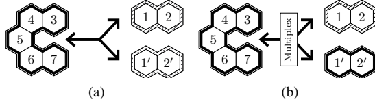
Figure 3: Runtime Configurations. (a) Replicated FMP (modules 1 and 2), with different FMP-Es. (b) Sampled FMP .
