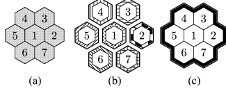
Figure 1: Modules, Fracturings, FMPs, and FMP-Es. (a) is a visualization of the application’s source code divided into modules. (b) and (c) are two different fracturings, i.e., visualizations of the application at runtime. The fracturing in (b) has maximum runtime isolation and consists of 7 FMPs, each using a different FMP-E. (c) is minimal isolation, with a single FMP and FMP-E.
