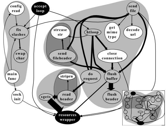
Figure 5: Module Interaction Graph for nhttpd-Latency. Black nodes are non-restartable modules; grey and white are restartable; edge thickness represents module interaction. For example, resources wrapper interacts heavily with sgets , and little with sock init . Seven modules (eg: dir list ) that are not executed in this workload are omitted. Shaded regions are module clusters used in intelligent fracturings; for isolating a grey module, the containing innermost cluster is placed in an FMP; for white modules, SMI is chosen. The inset shows the manually optimized partition for send file : two FMPs, each a shaded region (duplicated modules overlap both regions).
