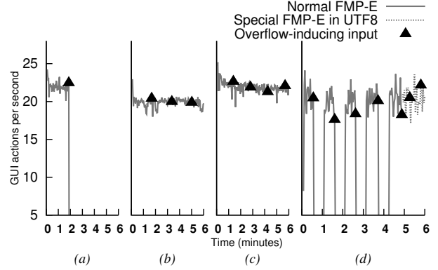
Figure 6: Pidgin: Tolerating Buffer Overflows. (a) Unmodularized. (b) Unmodularized with special environment. (c) UTF8 SMI with special FMP-E. (d) Adaptive fracturing.
