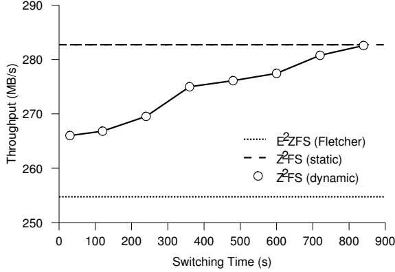
Fig. 9: Webserver Throughput with Different t_{switch} . This figure illustrates the throughput changes of webserver as t_{switch} increases. The dashed line and dotted line represent the throughput of webserver on Z 2 FS (static) and E 2 ZFS (Fletcher) respectively. The runtime of the webserver workload is 720 seconds.
