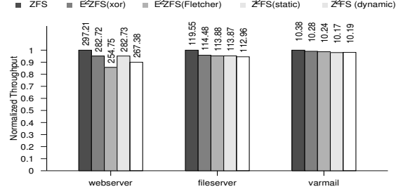
Fig. 8: Macro Benchmark. This figure shows the throughput of our macro benchmarks on ZFS, E 2 ZFS, Z 2 FS (static), and Z 2 FS (dynamic). Each workload runs for 720 seconds. Z 2 FS (dynamic) has t_{switch} = 92 seconds.
