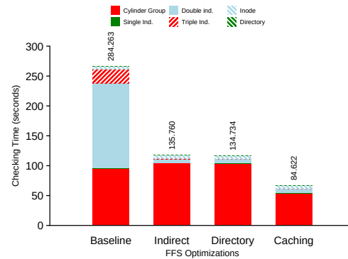
Fig. 21. FFS Fsck Duration By Block Type. Time required to run fsck on FFS using different levels of optimization, broken down by block type. “Single Ind.” refers to time spent reading the first indirect block for each file. “Double Ind.” and “Triple Ind.” refer to time spent reading the double and triple indirect blocks for each file, as well as their children. The numbers atop the bars indicate total duration.
