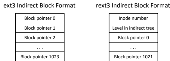
Fig. 5. Indirect Block Layout. This figure shows how the indirect blocks of ext3 and rext3 differ.
