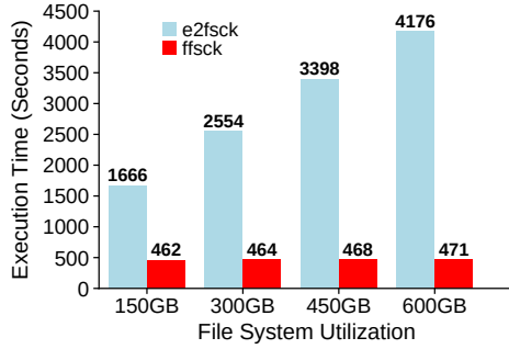
Fig. 10. E2fsck and ffsck Execution Time. Total running time of e2fsck and ffsck as file-system utilization increases.
