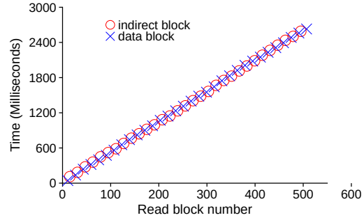
Fig. 16. Cumulative ext3 Strided Read Time. Cumulative time spent reading different block types in ext3 for the strided read benchmark.
