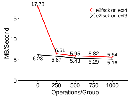
Fig. 3. e2fsck on Aging File System Images. This graph shows that e2fsck's speed degrades as the file system ages. The file system is on a 750 GB partition and has around 95% utilization.
