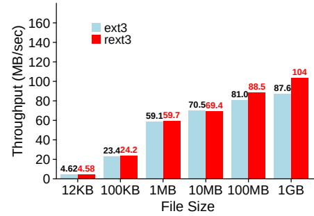
Fig. 14. Sequential Write Throughput. Sequential write throughput for a file of varying size.
