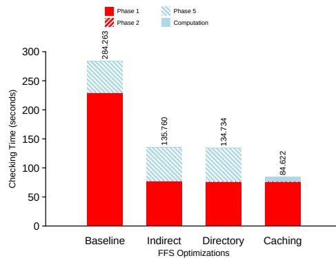
Fig. 20. FFS Fsck Duration By Phase. Time required to run fsck on FFS using different levels of optimization, broken down by I/O time in each phase, along with pure computation time (only a factor in the caching experiment). The numbers atop the bars indicate total duration.
