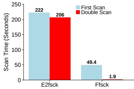
Fig. 12. Double Scan Execution Time. Total running time of e2fsck and ffsck in the presence of a doubly-allocated block.
