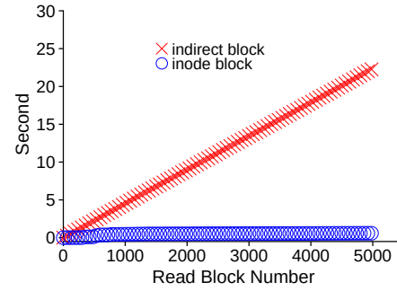
Fig. 2. Cumulative e2fsck Read Time In Phase 1. This figure shows the cumulative time to access each indirect block and inode block in phase 1 of e2fsck's scan.
