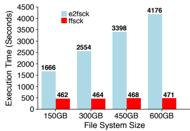
Figure 9: E2fsck and fsck Execution Time. Total running time of e2fsck and fsck as the file-system size increases.
