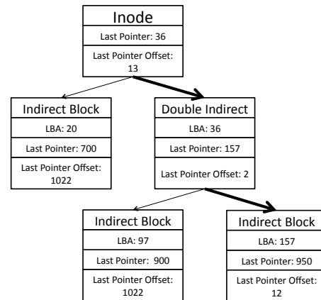
Figure 5: File Size Verification. This figure shows the logical tree structure used to verify a file's size. The bold arrows indicate the path followed to retrieve and construct the final offset set.
