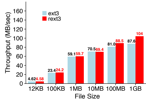
Figure 13: Sequential Write Throughput. Sequential write throughput for a file of varying size.
