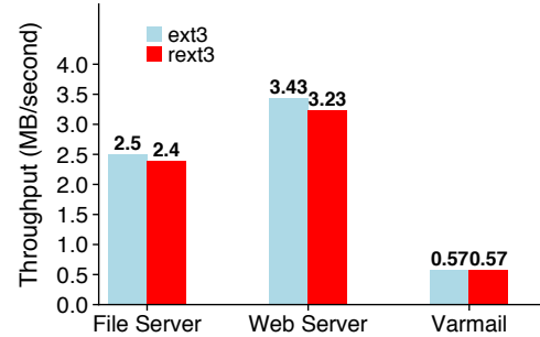
Figure 18: Filebench Performance. Performance of fileserver, webserver and varmail macrobenchmarks with ext3 and rext3.
