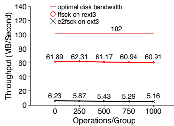
Figure 10: E2fsck and fsck Throughput Under Aging. Rate at which e2fsck and fsck scan a 750 GB file system as the file system ages.
