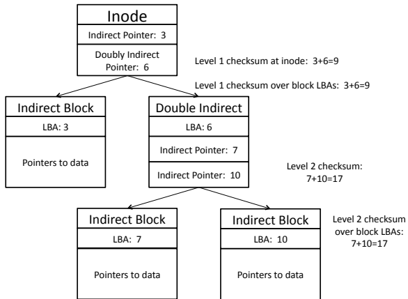
Figure 6: Checksum of Each Indirect Layer. This figure shows how ffsck calculates and verifies the checksum of each layer in the tree of indirect blocks.
