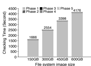
Figure 1: e2fsck Execution Time By Size. This graph shows e2fsck 's execution time for differently sized file-system images, broken down by time spent in each phase.
