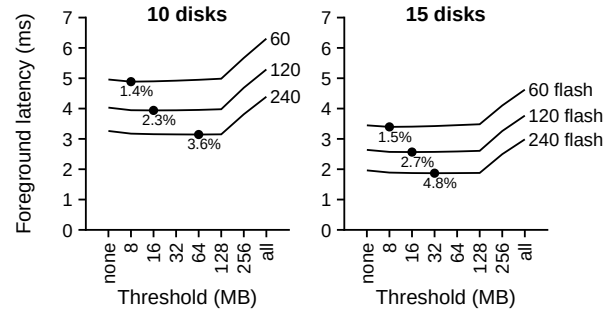
Figure 14: Flash Buffer. We measure how different file-buffering policies impact foreground requests with two plots (for 10 or 15 disks) and three lines (60, 120, or 240GB of flash). Different points on the x-axis represent different policies. The optimum point on each line is marked, showing improvement relative to the latency when no buffering is done.
