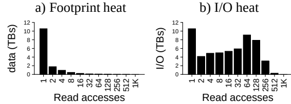
Figure 8: Read heat. In both plots, bars show a distribution across different levels of read heat ( i.e. , the number of times a byte is read). The left shows a distribution of the dataset (so the bars sum to the dataset size, included deleted data), and the right shows a distribution of I/O to different parts of the dataset (so the bars sum to the total read I/O).
