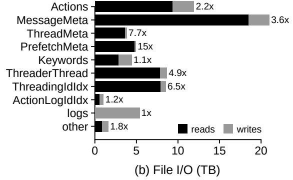
Figure 4: File types. Left: all accessed HDFS file data is broken down by type. Bars further show whether data was read, written, or both. Right: I/O is broken down by file type and read/write. Bar labels indicate the I/O-to-data ratio.
