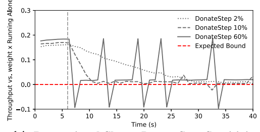
Figure 14: Proportional Share: DonateStep Sensitivity Analysis. We use the same setup as in Figure 11 when B is write-heavy. This figure shows A, the donor's throughput over time with different DonateStep.
