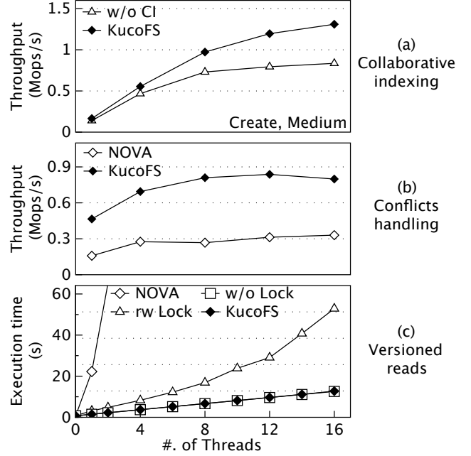
Figure 8: Benefits of collaborative indexing and versioned read . w/o CI: KucoFS without collaborative indexing.
