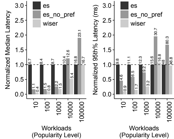
Figure 14: Single Term Matching Latency The latency (ms) is normalized to the median latency of Elasticsearch with default prefetching.
