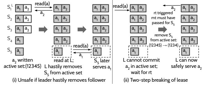
Figure 4: Active Set and Leases. (i) shows how removing a follower hastily can expose non-monotonic states; (ii) shows how ORCA breaks leases.
