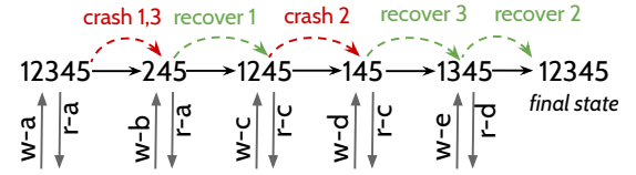
Figure 9: An Example Failure Sequence. The figure shows an example sequence generated by our test framework.
