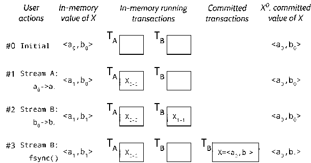
Figure 2: Hybrid-granularity Journaling. Timeline showing hybrid-granularity journaling in ccfs. Block X initially contains the value \langle a_0, b_0 \rangle . T_A and T_B are the running transactions of streams A and B ; when B commits, X is recorded at the block level on disk.
