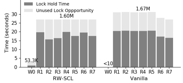
Figure 11. Comparison of RW-SCL and KyotoCabinet The dark bar shows the lock hold time for each individual thread and the light bar shows the lock opportunity not being unused. The values on top of the bar shows the aggregated throughput (operations/sec) for the writer and reader threads.
