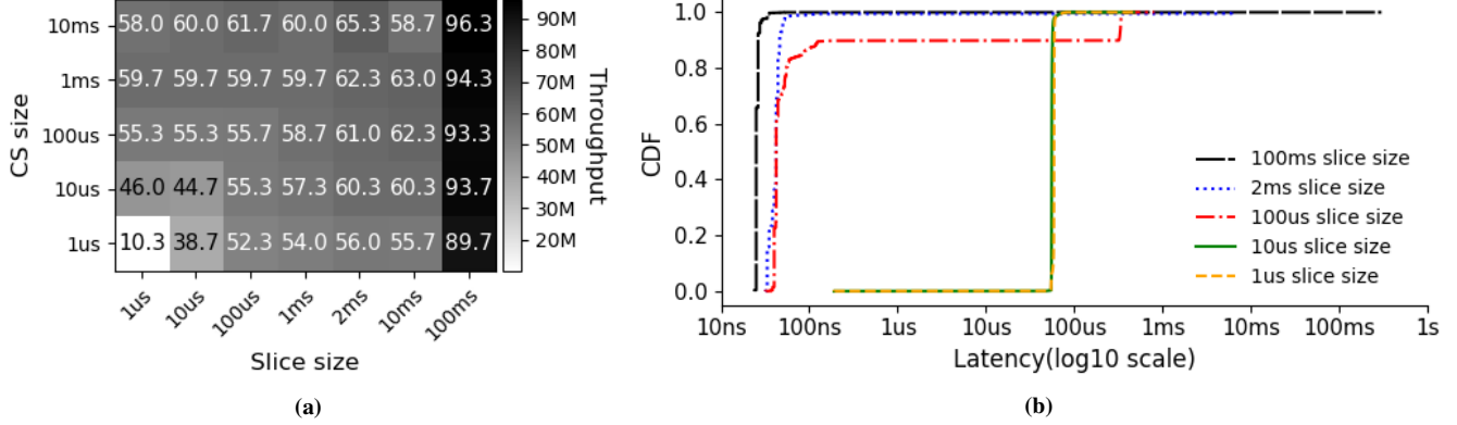
Figure 8. Impact of lock slice size on performance. The left figure (a) shows the throughput across two dimensions : critical section and the slice size. The right figure (b) shows the wait-time distribution when the lock slice varies and the critical section size is 1\mu s .
