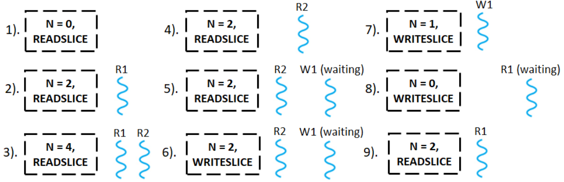
Figure 4. Reader-Writer Scheduler-Cooperative Locks. In (1) The lock is initialized and free. (2) A reader thread R1 acquires the lock and continues its execution in the critical section. (3) Another reader thread R2 also joins in. (4) Reader R1 leaves the critical section. (5) A writer thread W1 arrives and waits for the write slice to start. (6) Write slice is started and W1 waits for reader R2 to release the lock. (7) Reader R2 releases the lock and writer W1 acquires the lock. (8) Reader R1 now arrives again and waits for the read slice to start. (9) W1 releases the lock and the read slice starts allowing the reader R1 to acquire the lock.
