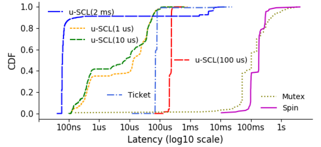
Figure 9. Interactivity vs. Batching. The figure shows the comparison of the wait-time to acquire the lock for mutex, spinlock, ticket lock and u-SCL.
