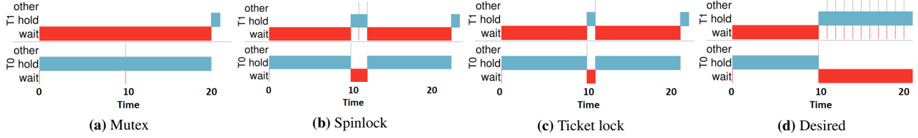
Figure 2. Impact of Critical Section Size. The behavior of existing locks when the critical section sizes of two threads differ are shown. The CFS scheduler is used and each thread is pinned on a separate CPU. “wait” represents the time spent waiting to acquire the lock; “hold” represents the critical section execution, i.e., the time the lock is held; “other” represents the non-critical section execution.
