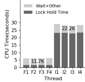
Figure 1. Scheduler subversion with UpScaleDB. We use a modified built-in benchmarking tool ups_bench to run our experiments. Each thread executes either find or insert operations and runs for 120 seconds. All threads are pinned on four CPUs and have default thread priority. “F” denotes find threads while “I” denotes insert threads. “Hold” represents the critical section execution, i.e., the time the lock is held; “Wait + Other” represents the wait-times and non-critical section execution. The value presented on the top of the dark bar is the throughput (operations/second).
