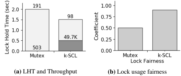
Figure 14. Rename Lock Comparison. The figure presents a comparison of two locks – mutex and k-SCL for 2 threads on two CPUs; each has the same thread priority and one thread is performing rename operations on a directory that is empty while another thread is performing rename on a directory having a million empty files.
