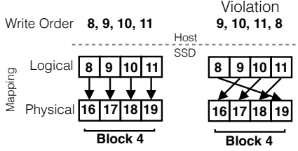
Figure 1: Example of Aligned Sequentiality and a violation of it. Each block has four pages. Writes must be programmed on a flash block from low to high pages to avoid program disturbance. The page-level mapping on the left can be converted to a single block-level mapping: logical block 2 \rightarrow physical block 4. The example on the right cannot be converted without re-arranging the data.
