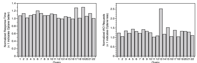
(a) Response Time (b) Normalized Number of I/O Requests Figure 1: Normalized TPC-H Response Time and Number of I/O Requests, Optane SSD vs. Flash SSD
