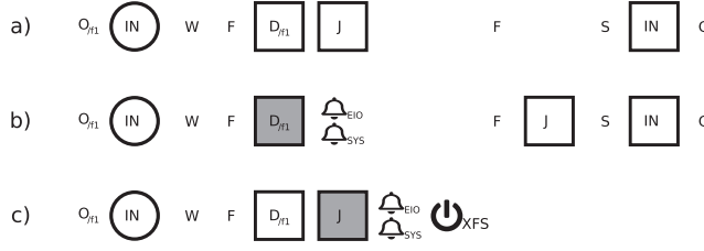
Fig. 6. Blockviz traces for w_{su} on XFS:
