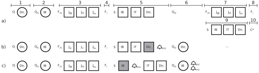
Fig. 4. Blockviz traces for w_{dir} on ext4 ordered mode:
