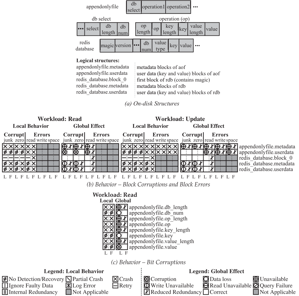
Fig. 2. Redis. (a) The on-disk format of the files and the logical data structures of Redis. The logical structures take the following form: file_name.logical_entity . If a file can be contained in a single file-system block, then we do not show the logical entity name. (b) System behavior when corruptions (corrupted with either junk or zeros), read errors, write errors, and space errors are injected in various on-disk logical structures in Redis. Within each system workload (read and update), there are two boxes—first, local behavior of the node where the fault is injected and, second, clusterwide global effect of the injected fault. The rightmost annotation shows the on-disk logical structure in which the fault is injected. Annotations on the bottom show where a particular fault is injected (L, leader/master; F, follower/slave). A gray box for a fault and a logical structure combination indicates that the fault is not applicable for that logical structure. For example, write errors are not applicable for any data structures in the read workload (since they are not written) and hence shown as gray boxes. (c) The behavior when bit corruptions are injected. For bit corruptions, we flip a single bit in a field within the on-disk structure. For example, appendonlyfile.db_num is part of appendonlyfile.metadata . The legend at the bottom is common to both (b) and (c).
