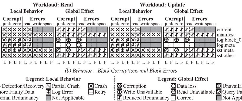
Fig. 10. CockroachDB. (a) The on-disk format of the files and the logical data structures of CockroachDB. (b) System behavior when faults are injected in various on-disk logical structures.
