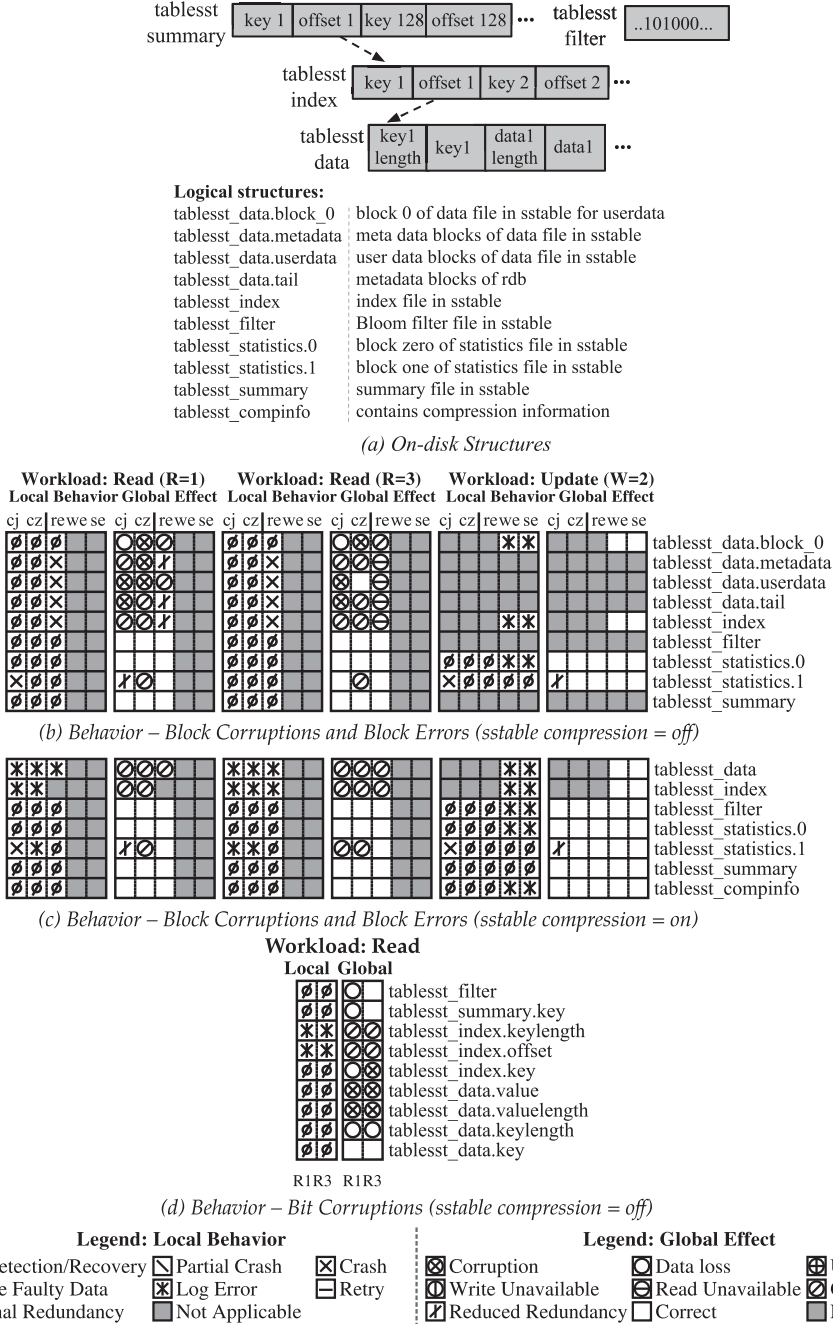
Fig. 5. Cassandra. (a) The on-disk format of different structures in Cassandra. (b) and (c) System behavior in the presence of block corruptions (corrupted with either junk (cj) or zeros(cz)), read errors (re), write errors (we), and space errors (se) when sstable compression is turned off and turned on, respectively. (d) The behavior in the presence of bit corruptions when sstable compression is off; the annotations on the bottom indicate the read quorum (R1, quorum of 1; R3, quorum of 3).
