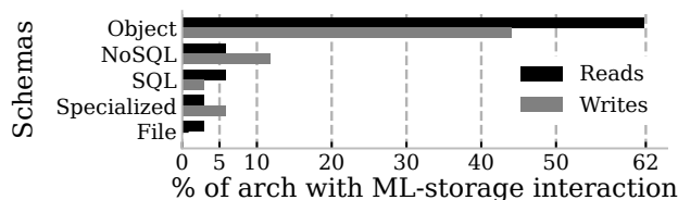
(b) Popularity of storage services that interact with ML services. The distribution is normalized against the number of architectures having at least one ML service interacting with any storage service.
