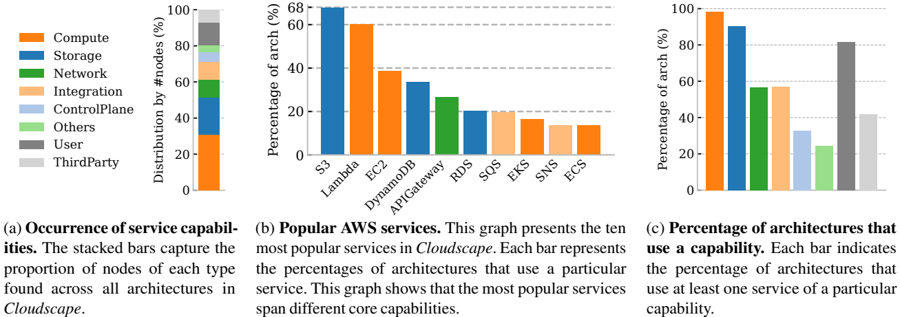
Figure 3: Composition of Architectures.
