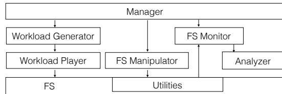
Figure 2: Chopper components.
