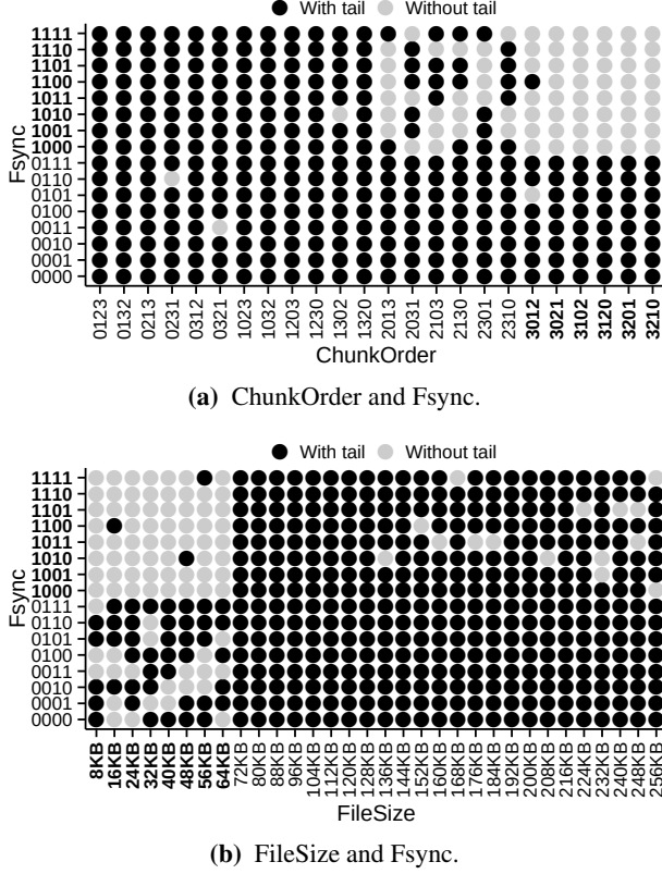
Figure 6: Tail Runs in the Interactions of Factors Note that each interaction data point corresponds to multiple runs with other factors varying. A black dot means that there is at least one tail case in that interaction. Low-danger zones are marked with bold labels.
