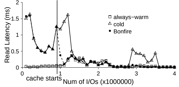
Figure 13: Read latency of Day 5 and 6 of proj1
