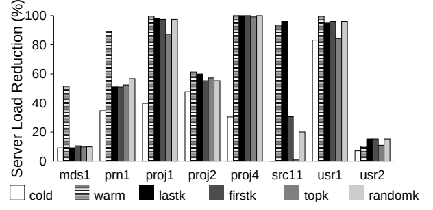
Figure 7: Server I/O Load Reduction
