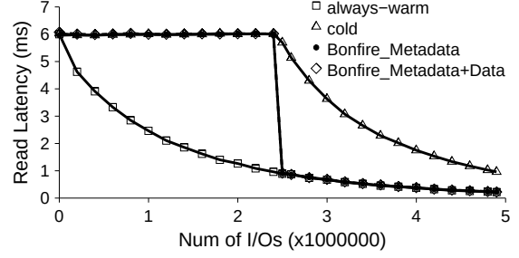
Figure 11: Read latency of the Zipf workload
