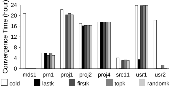
Figure 6: Convergence Time
