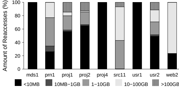
Figure 3: Reuse Distance
