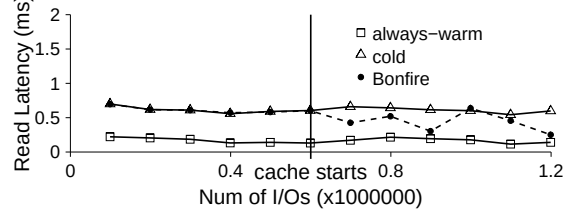
Figure 15: Read latency of Day 5 and 6 of web2
