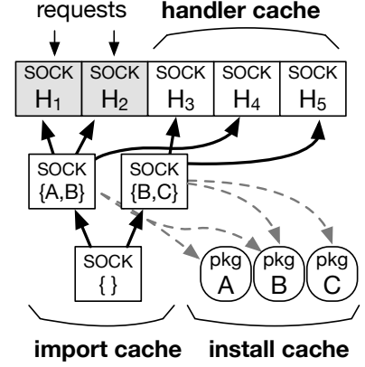
Figure 12. Serverless Caching
