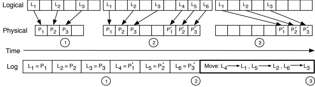
Figure 3: Transactions via address remapping By using an application-managed scratch area, atomic transactional updates can be implemented using range operations. At ① the system is in its consistent pre-transaction state, with logical blocks L_1 , L_2 , and L_3 each mapped to blocks containing the initial versions of the relevant data. Between ① and ②, new versions of these blocks are written out and mapped to logical addresses in a temporary scratch area ( L_4 , L_5 , and L_6 ). Note that this portion is not required to proceed atomically. Once the temporary locations have all been populated, an atomic range-move operation remaps the new blocks at L_4 , L_5 , and L_6 to L_1 , L_2 , and L_3 , respectively, leading to ③, at which point the transaction is fully committed.
