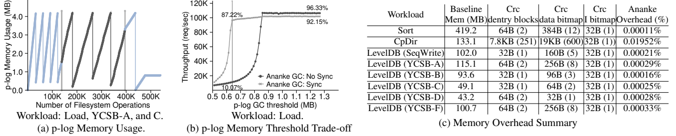
Figure 9: Memory Usage (LevelDB). In (c), the amount of Baseline Mem includes: one is the difference between the amount of memory in the data segment (heap) before and after running each workload; the second is the in-memory file system structures (corresponding to disk, including data blocks and metadata blocks); Overhead is calculated using the CRC memory added.
