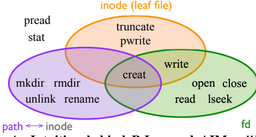
Figure 4: Intuition behind P-Log and AIM We enumerate POSIX APIs and categorize them according to how filesystem abstractions are updated. Representative ones are shown for brevity; mmap , chown , and chmod are excluded.
