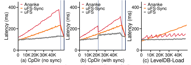
Figure 10: Restart time with uFS, uFS-Sync, and Ananke. The light blue vertical lines indicate the time where a background sync occurs; the deep blue (last) vertical lines indicate a checkpoint. X-axis is the timing (# of ops) of a p-crash.
