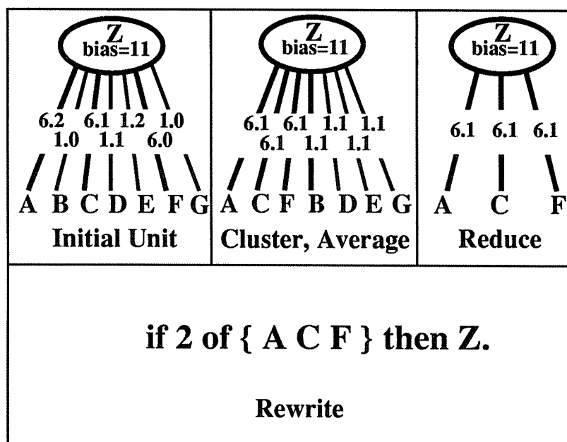
Figure 6. A sketch of the NofM rule-extraction algorithm.
