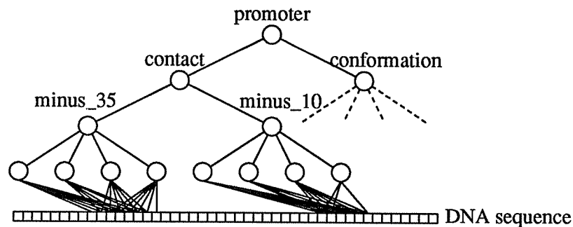
Figure 7. The initial neural network for promoter recognition that KBANN produces.
