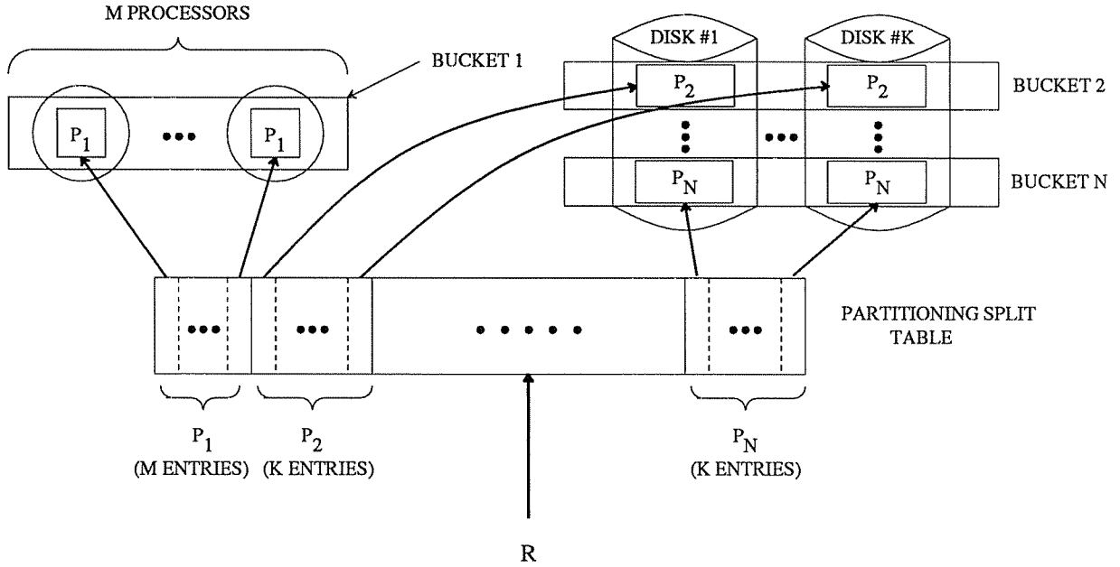
Partitioning of R into N logical buckets for Hybrid hash-join. Figure 8
