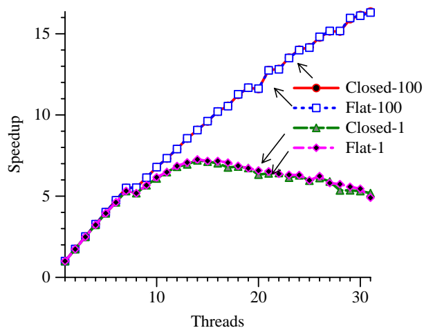
Figure 8: Scalability of B-Tree using Flat Closed Nesting and Closed Nesting with Partial Aborts and 1 (Flat-1 and Closed-1) or 100 (Flat-100 and Closed-100) free lists
